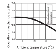
Temperature compensation curve
