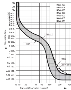
■ Operating characteristic curves
