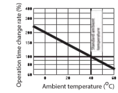
■ Temperature compensation curve
