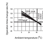
Temperature compensation curve
