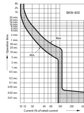
Operating characteristic curves
