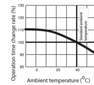
Temperature compensation curve
