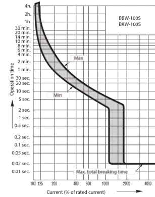
■ Operating characteristic curves
